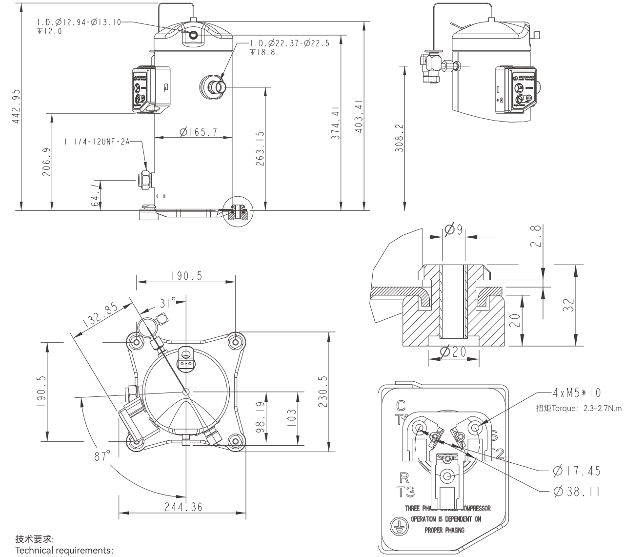
接线盒布置 Junction Box Layout
