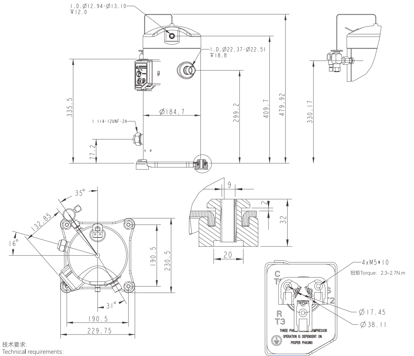
接线盒布置 Junction Box Layout
